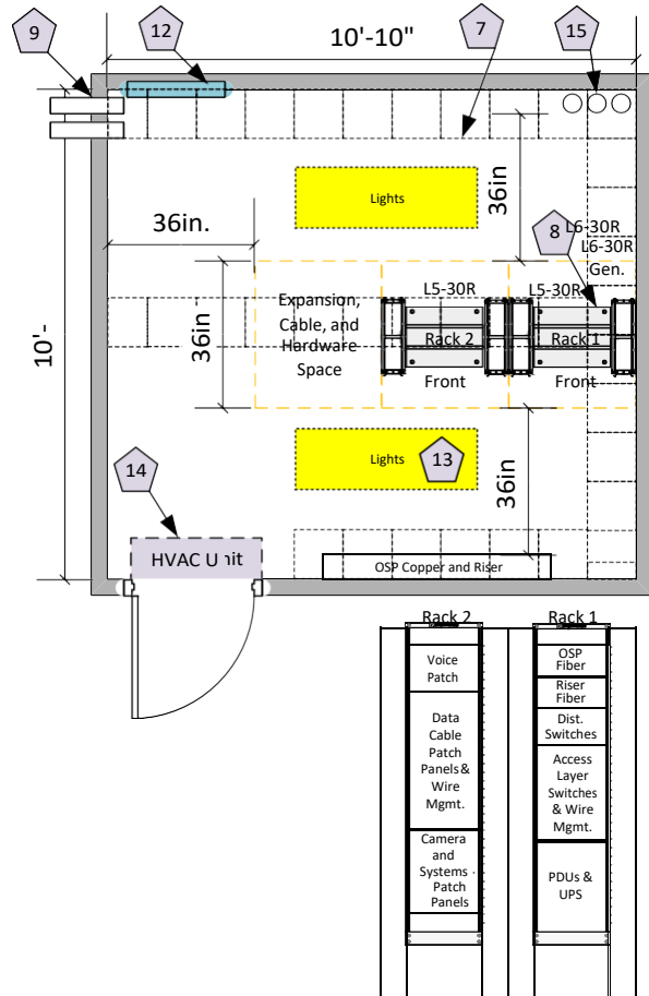
Exhibit 2 - 2 Rack MDF
