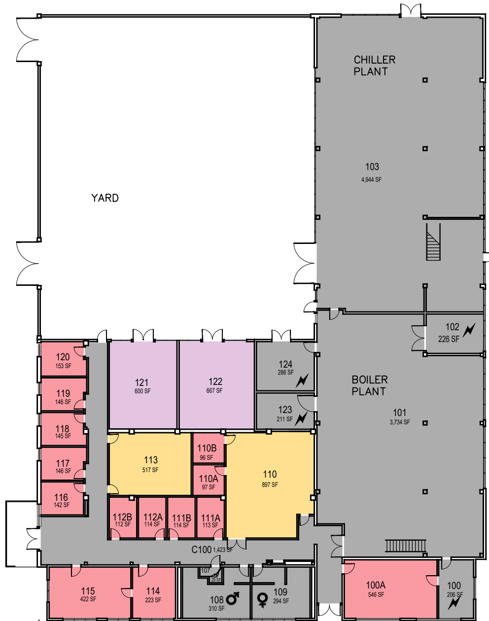
First Floor
