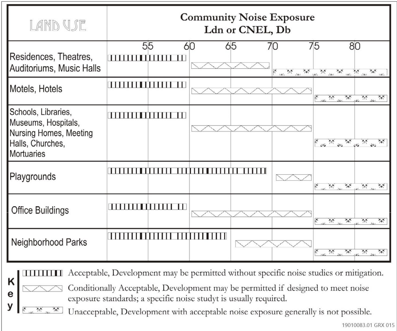
Figure 3.10-1 Noise Exposure
