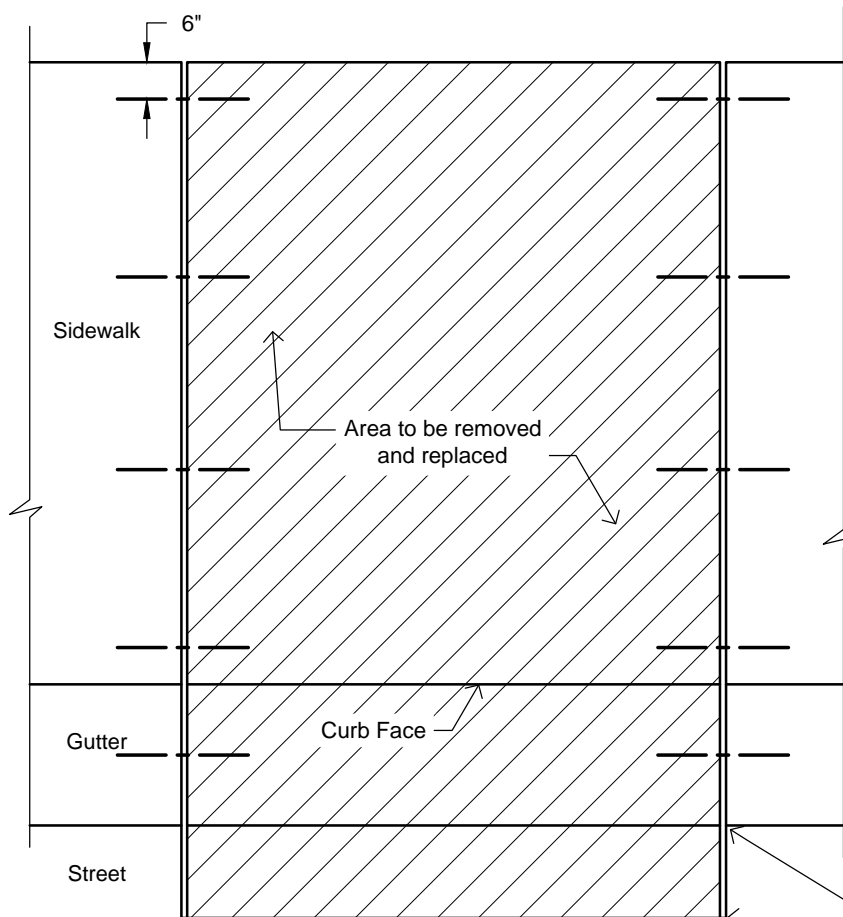
SIDEWALK SECTION
