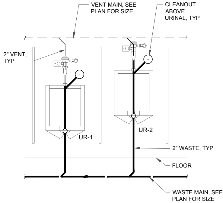
ELEVATION VIEW
