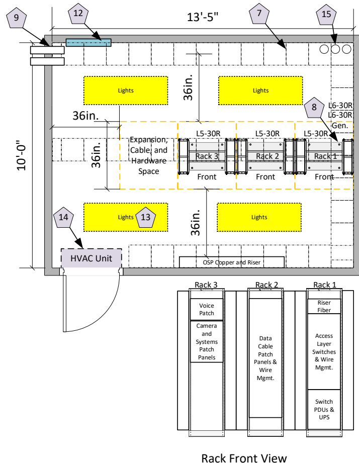
Exhibit 7 - 3 Rack IDF
