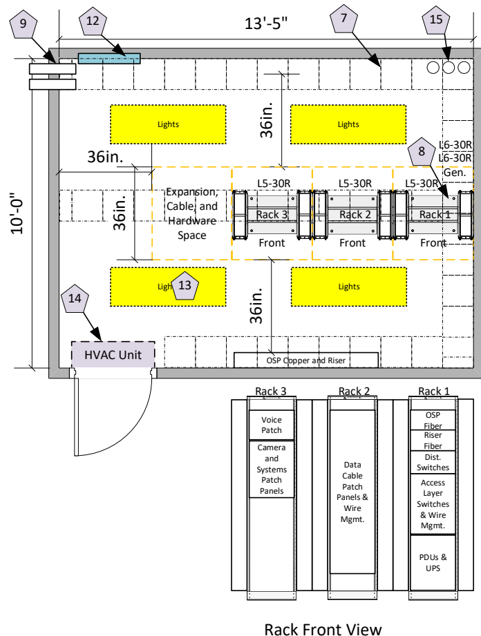
Exhibit 3 - 3 Rack MDF
