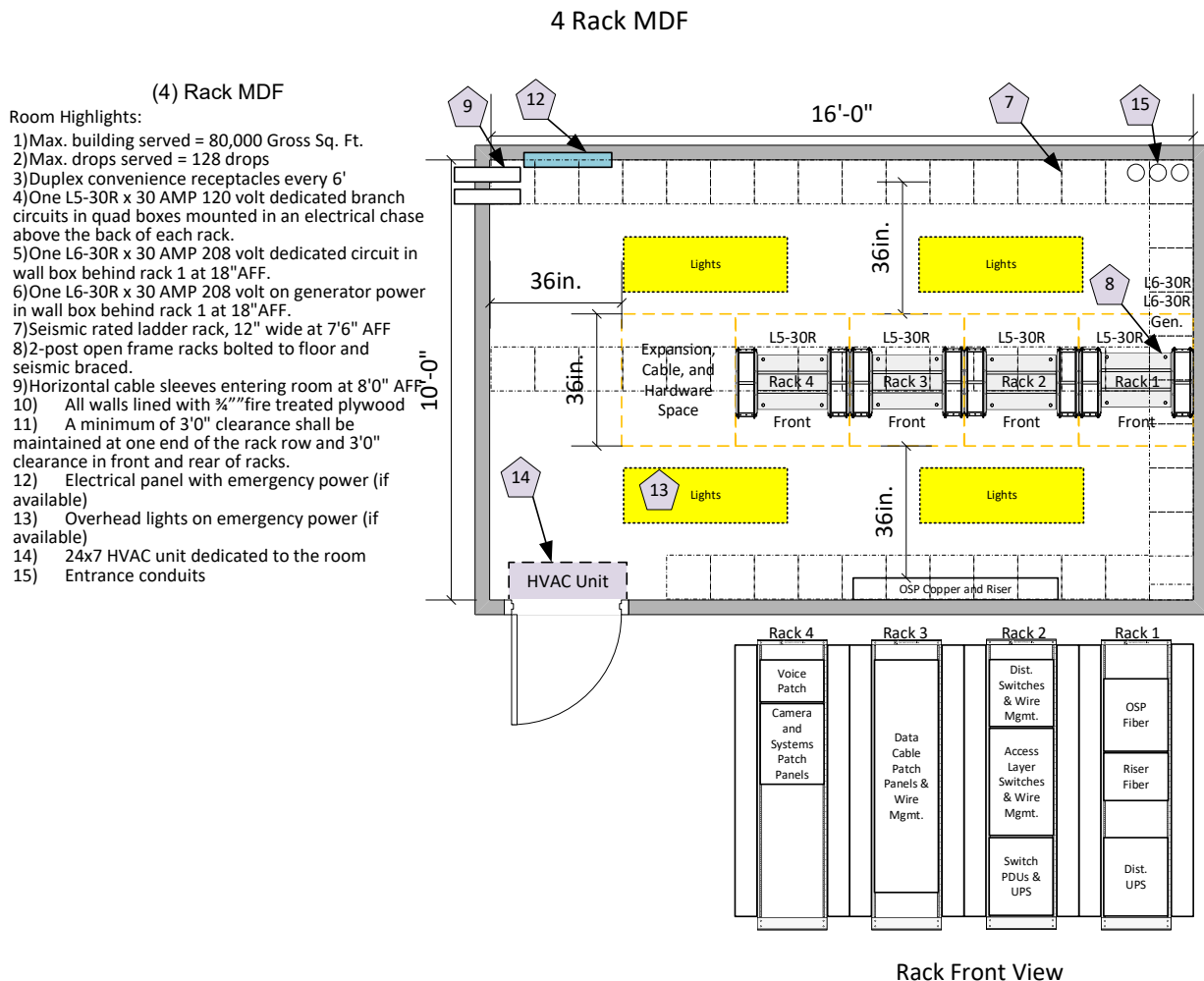
Exhibit 4 - 4 Rack MDF
