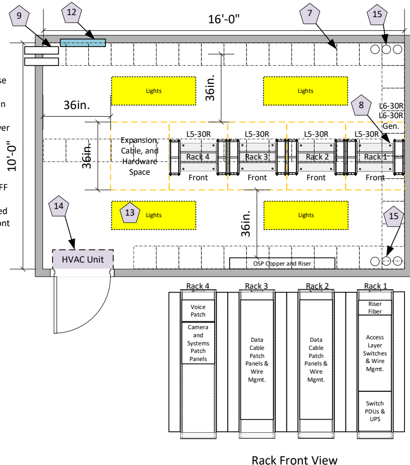
Exhibit 8 - 4 Rack IDF
